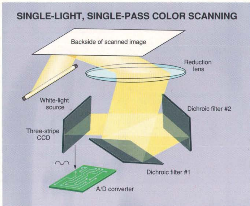
Figure 3: Dichroic filters separate white light into its primary color components. Each separated color shines onto a row of a three-stripe CCD.
